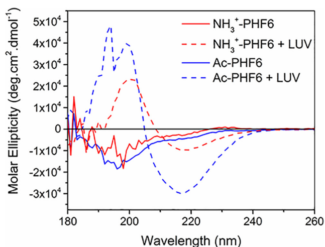
Figure 10. CD spectra of 168 \mu\text{g/ml} of \text{NH}_3^+ -PHF6 and Ac-PHF6 peptides alone (solid line) and in the presence LUVs (688 \mu\text{M} lipids, 70 mol % POPC and 30 mol % POPG) after 1 h incubation at room temperature (dashed line). LUVs caused the largely random coil peptides to adopt \beta -sheet-rich structures.
