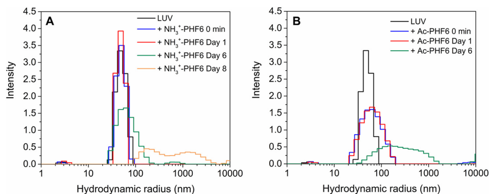
Figure 11. Size distribution of LUVs (20 \mu\text{M} lipids, 70 mol % POPC and 30 mol % POG) incubated at room temperature in the presence of 50 \mu\text{g}/\text{ml} of \text{NH}_3^+ -PHF6 (A) or Ac-PHF6 (B) over time as detected by DLS. LUVs size distribution was unchanged after 1 day of incubation with \text{NH}_3^+ -PHF6 and became larger after 6 days of incubation. In contrast, Ac-PHF6 induced a rapid increase of R_h and broader LUV size distribution immediately upon addition.
